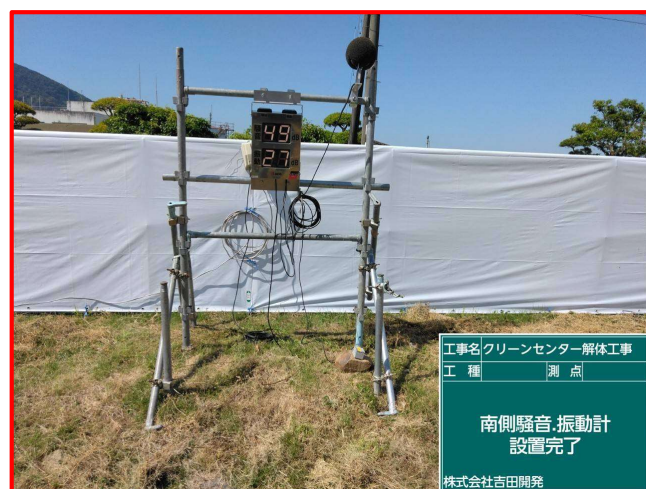
騒音・振動計② (南側)
